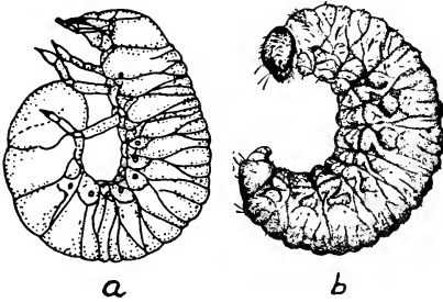
Fig. 25. Larvae: a, Anomala kansana Hayes & McColloch; b, clover leaf weevil, Hypera punctata (Fab.)
